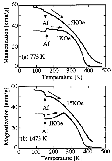
FIG. 4. Thermomagnetization curves in the magnetic fields of 1 and 15 kOe for Ni_{51}Fe_{22}Ga_{27} alloy annealed at (a) 773 K and (b) 1473 K.
