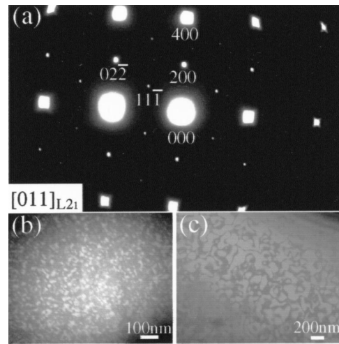
FIG. 3. (a) SAD pattern obtained from the alloy annealed at 773 K and TEM DFIs taken from \{111\}L_{21} reflection of the parent phase in Ni_{51}Fe_{22}Ga_{27} alloy annealed at (b) 1473 and (c) 773 K.
