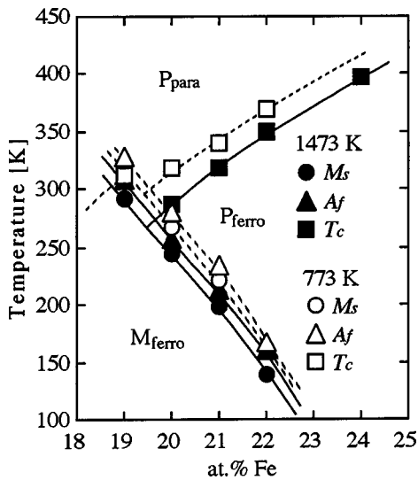
FIG. 1. Composition dependence of T_c , M_s , and A_f in Ni_{73-x}Fe_xGa_{27} annealed at 1473 and 773 K. The parent and the martensite phases are given by P and M, respectively.
