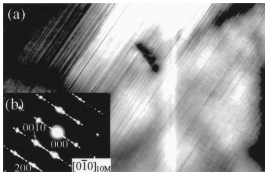
FIG. 2. (a) TEM bright-field image showing the typical microstructure and (b) the corresponding SAD pattern at 90 K taken from the martensite phase of Ni_{51}Fe_{22}Ga_{27} alloy annealed at 773 K.
